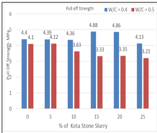
Fig. 5 Pull-off Strength (Water Cement Ratio =0.40 and 0.50)
