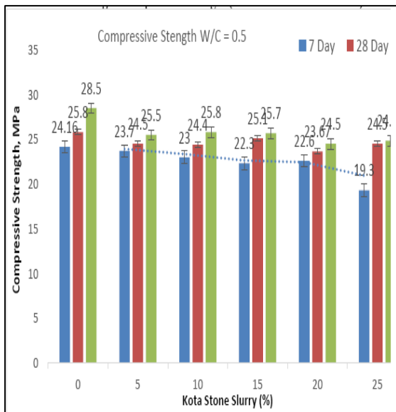
Fig 2: Compressive Strength (Water Cement Ratio = 0.50)
