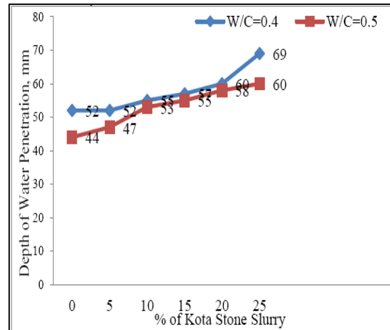
Fig. 6 Depth of Water Penetration, DIN 1048 Permeability Test (Water Cement Ratio = 0.40 and 0.50)
