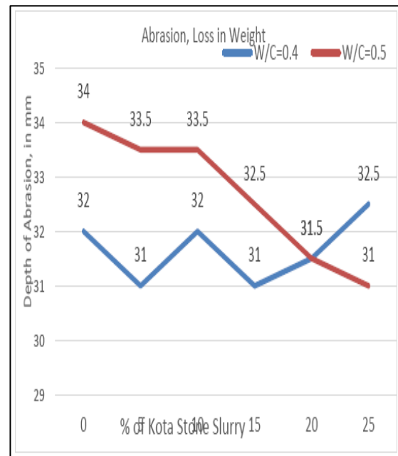
Fig 10: Depth of Abrasion, Abrasion Test
