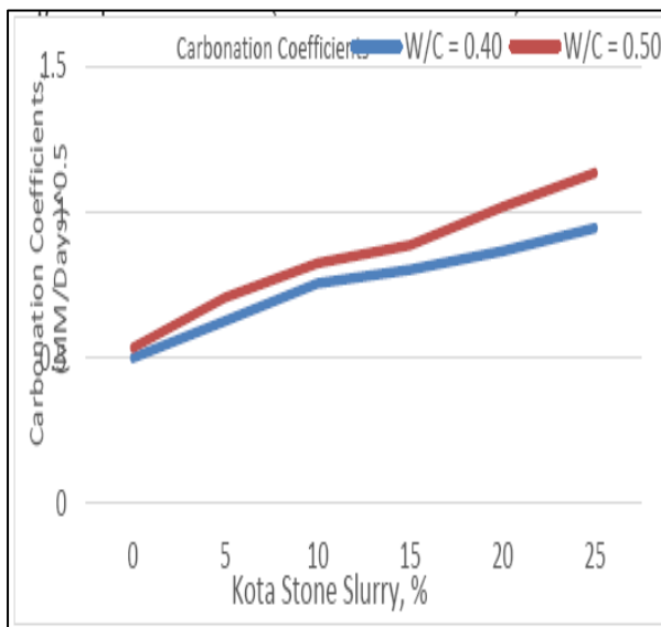
Fig 9: Carbonation Coefficients (Water Cement Ratio = 0.40 and 0.50)
