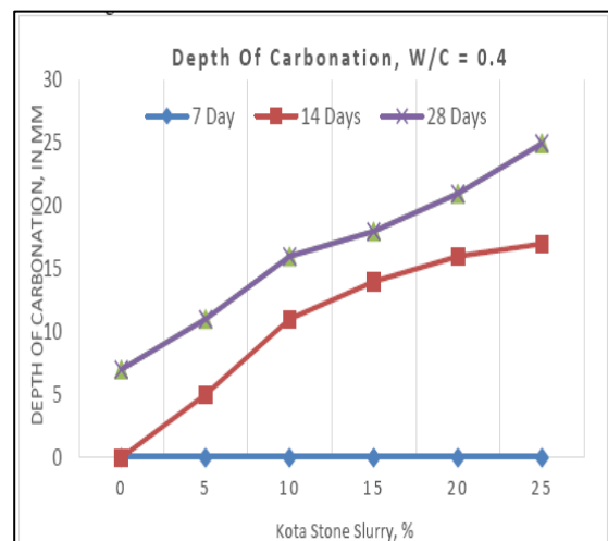
Fig 7: Depth of Carbonation (Water Cement Ratio = 0.40)
