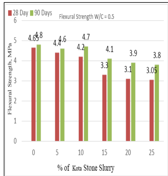
Fig 4 Flexural Strength (Water Cement Ratio = 0.50)
